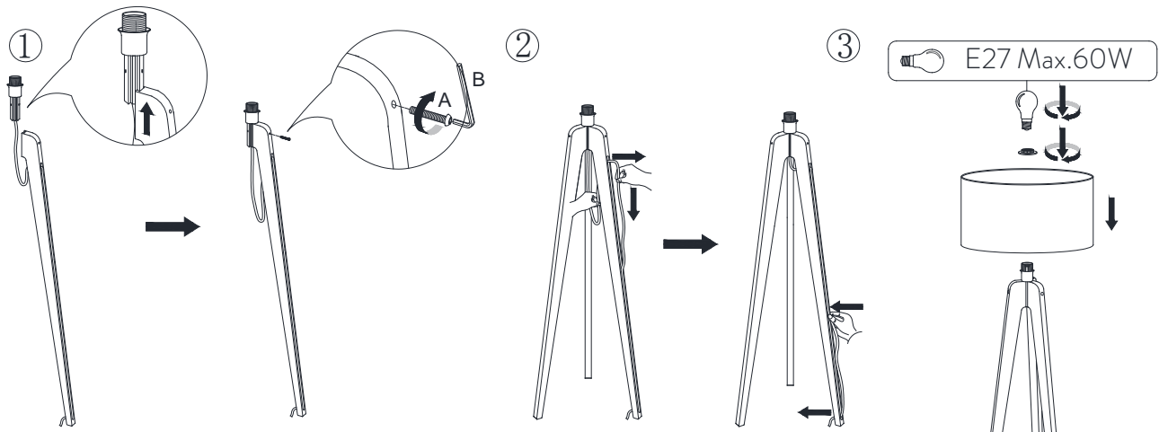
(A) Allen Bolt M6 x55mm x 3
